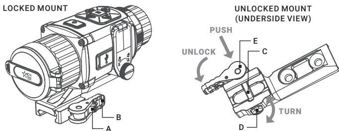
FIGURE 2-7. QUICK RELEASE MOUNT
