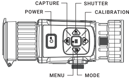
FIGURE 2-2. CONTROL BUTTONS
