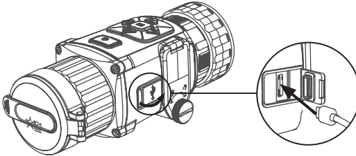
FIGURE 2-2. CABLE INTERFACE
