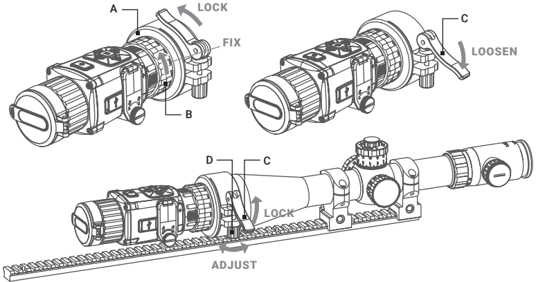
FIGURE 2-5. CLIP-ON INSTALLATION
