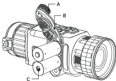
FIGURE 2-1. BATTERY INSTALLATION
