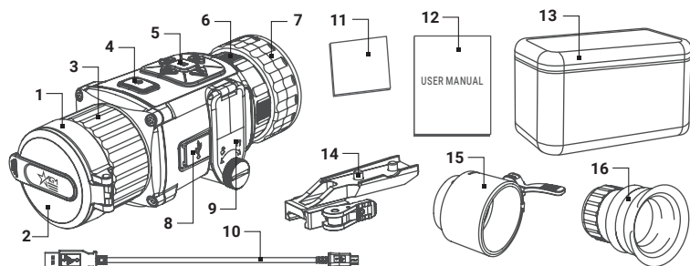
FIGURE 1-1. MAIN PARTS AND COMPONENTS
