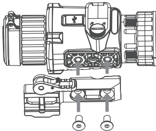
FIGURE 2-6. QUICK RELEASE MOUNT INSTALLATION
