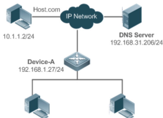
Figure 7-1 Dynamic Domain Name Resolution
