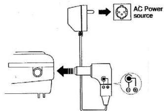
↑ Power Supply
